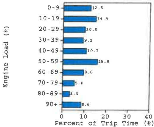
Engine Load Histogram
