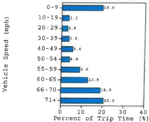
Vehicle Speed Histogram
