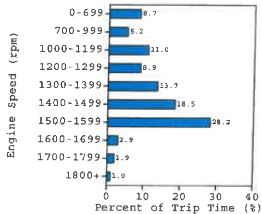
Engine Speed Histogram
